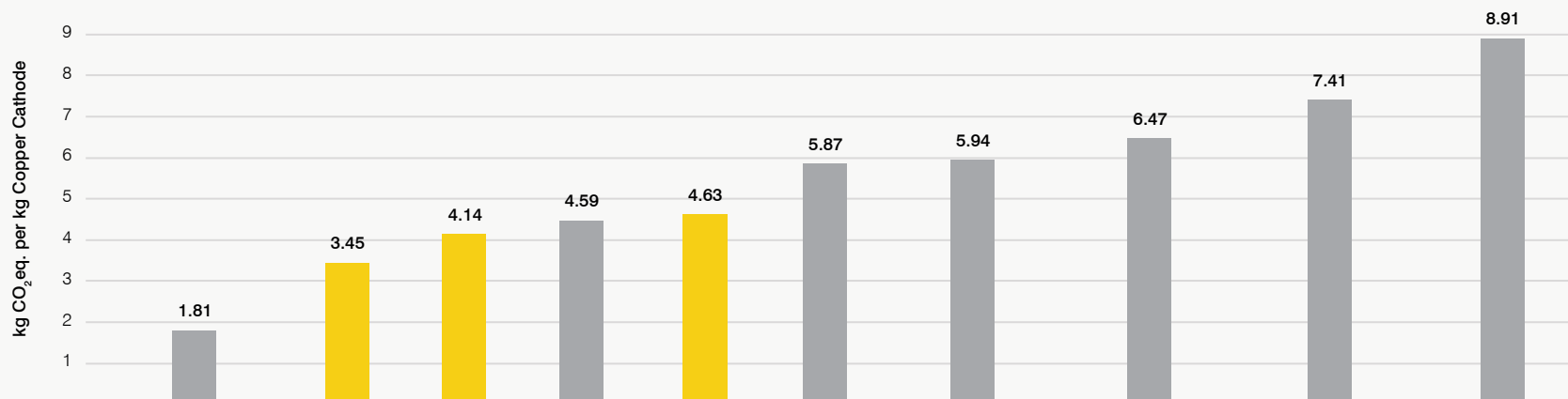
1kg Copper Cathode (99.99% Cu) – Climate Change Impact by processing technology and location
