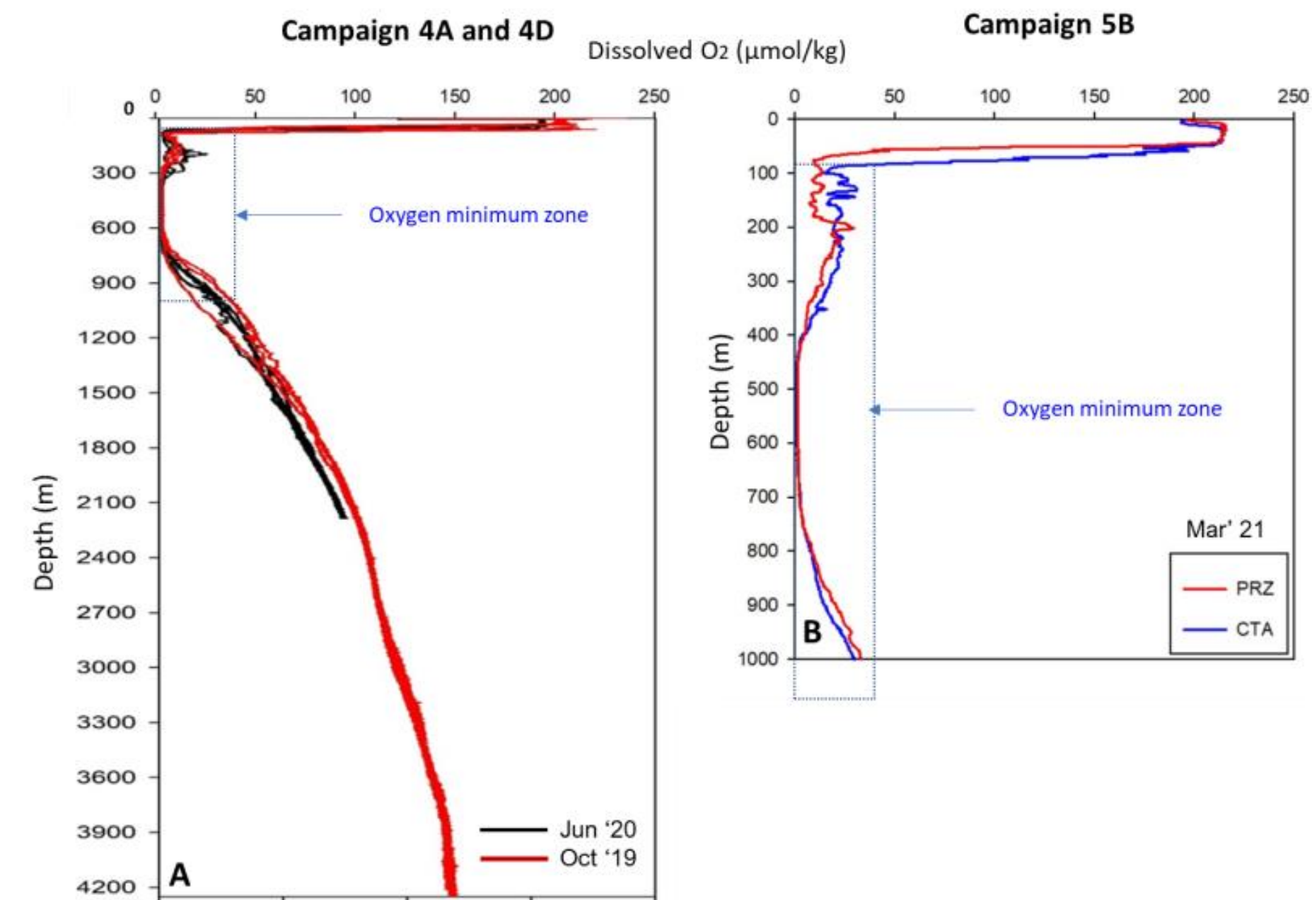
Figure 5-43. A - Dissolved Oxygen profiles measured on Campaigns 4A, 4D; B - Dissolved Oxygen profiles measured on Campaign 5B.
